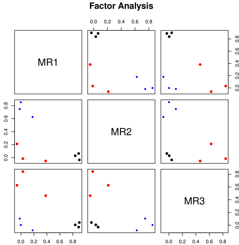
Figure 4: A graphic representation of the 3 oblique factors from the Thurstone data using plot . Factors were transformed to an oblique solution using the oblmin function from the GPArotation package.
