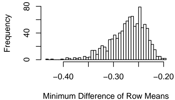
Python Null Distribution
