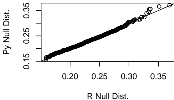
Maximum Difference of Row Means
