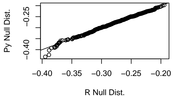
Minimum Difference of Row Means
